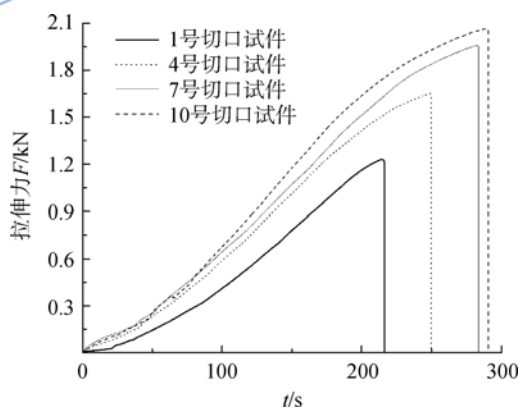
图4 切口试件拉伸结果 Fig. 4 Tensile test results of notched specimens
